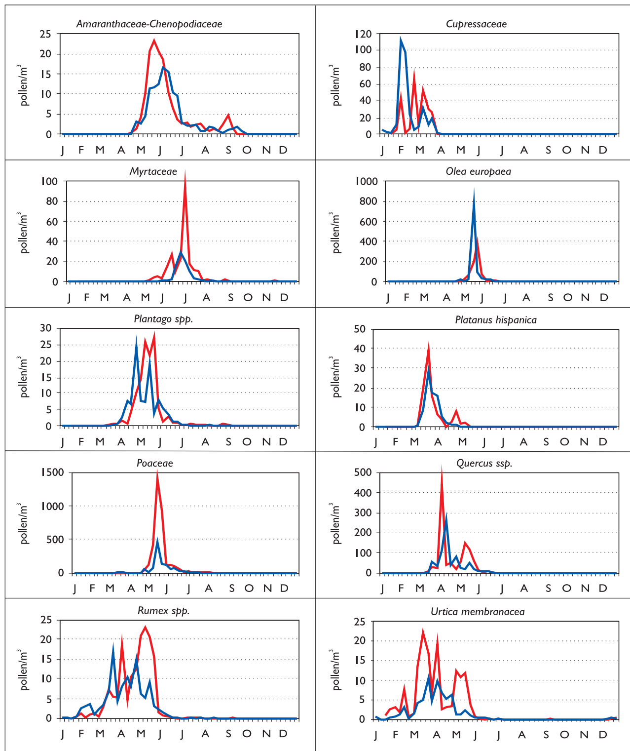
Figure 2. Weekly average pollen concentrations (pollen grains / m 3 ) for the main pollen types during 2003 and 2004
